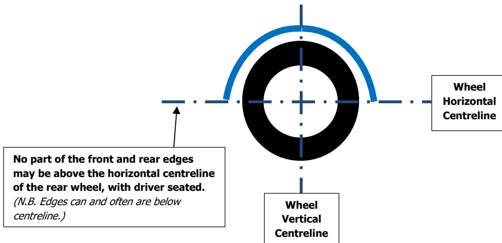
Rear Mudguard side view – Offside (Nearside is mirror view)
