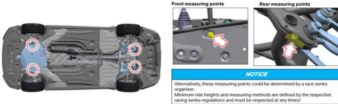
(Figures – Vehicle underbody and measurement points to determine ride height)
