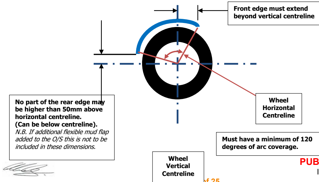
Front Mudguard side view – Offside (Nearside is mirror view)
